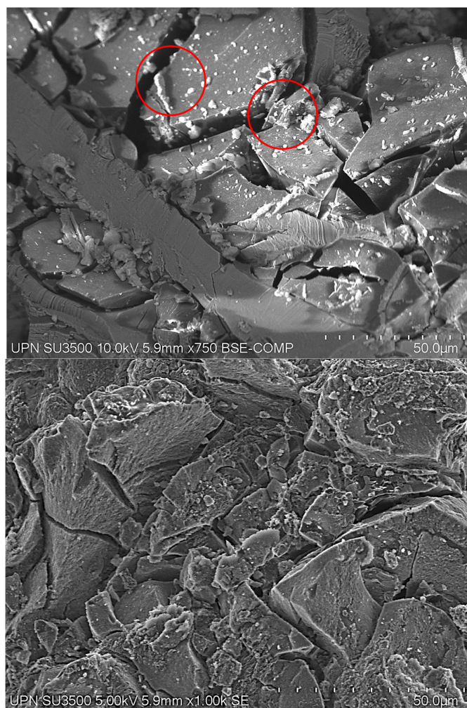
Figure 1. (A) Results of surface analysis of Biosilica-Humic acid with magnification x750 and (B) Biosilica-Humic acid with magnification x1000
