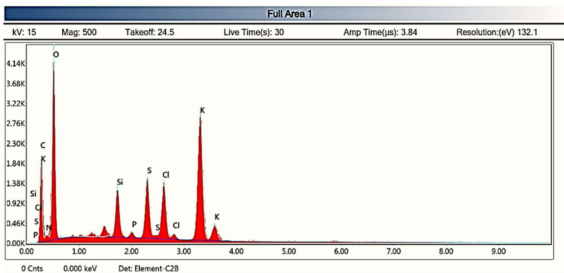
Figure 2. Graph of SEM-EDX chemical element analysis results in Biosilica-Humic Acid (BSi-AH)
