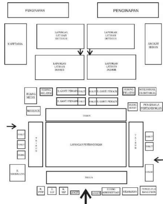
Gambar 7. Diagram Ruang
